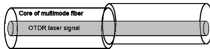
Figure 9. OTDRs only see the middle of the multimode fiber core
