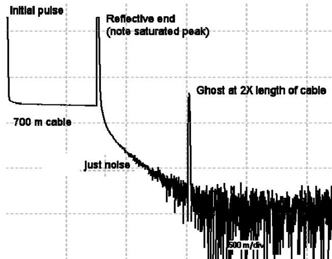
Figure 6. OTDR "ghosts"
