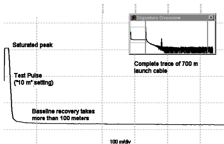
OTDR launch pulse and launch cable
